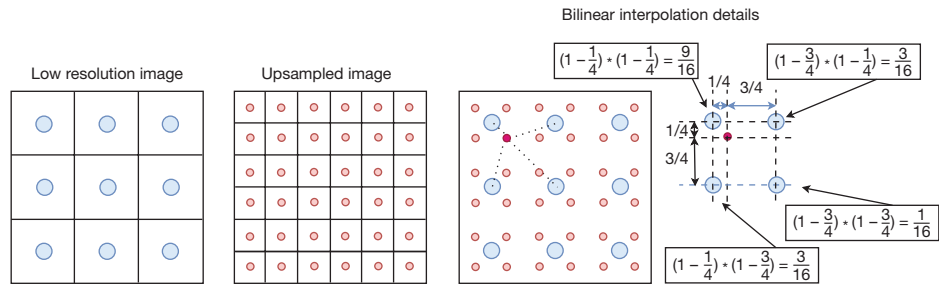
Figure B-9 2x upsampling
