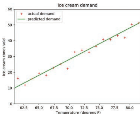
Figure A-1 Relationship between temperature and number of ice cream cones sold. For readers more familiar with the Celsius temperature scale, a rule of thumb is that 61°F is about 16°C and 82°F is about 28°C (just flip the digits).
