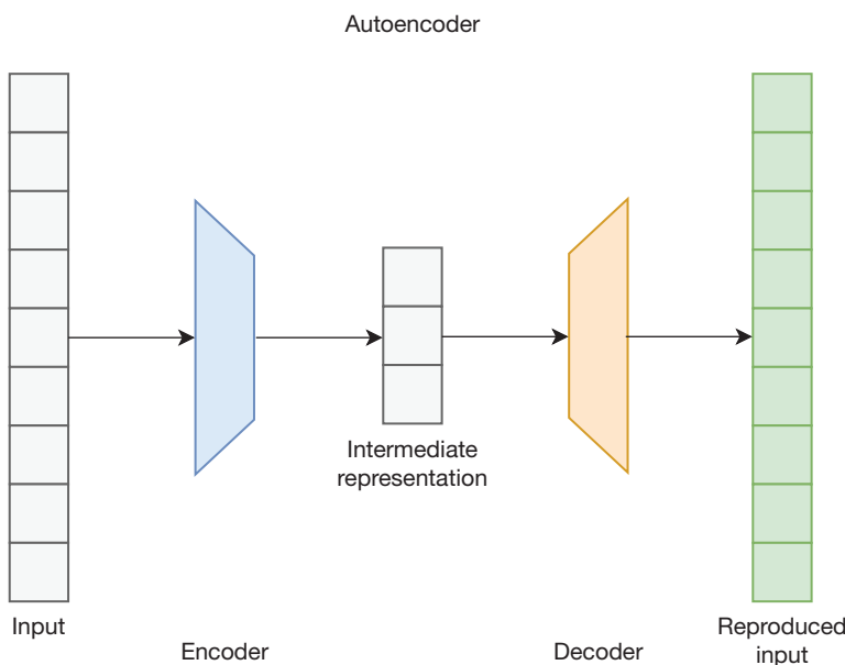
Figure 17-1 Autoencoder architecture
