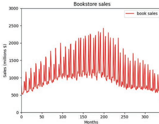
Figure 9-10 Historical bookstore sales from 1992 to 2020
