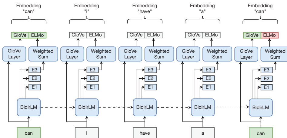
Figure C-7 Process of forming context-dependent embeddings by concatenating ELMo embeddings with any other context-independent embedding
