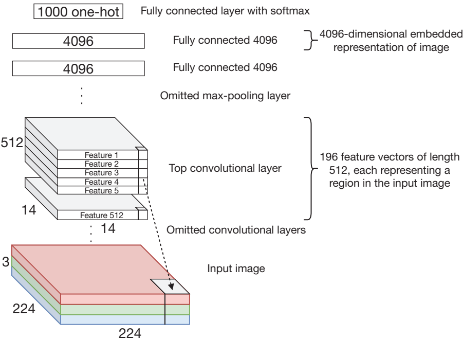
Figure 16-3 Simplified view of the VGG19 network where many layers have been omitted
