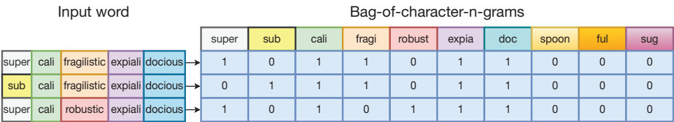
Figure C-1 Bag-of-n-grams based on some of the n-grams in the word supercalifragilisticexpialidocious and two variations on that word
