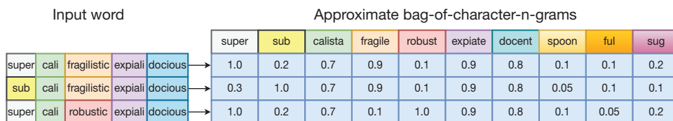
Figure C-2 Approximate-bag-of-n-grams where each vector entry indicates similarity to the target n-gram
