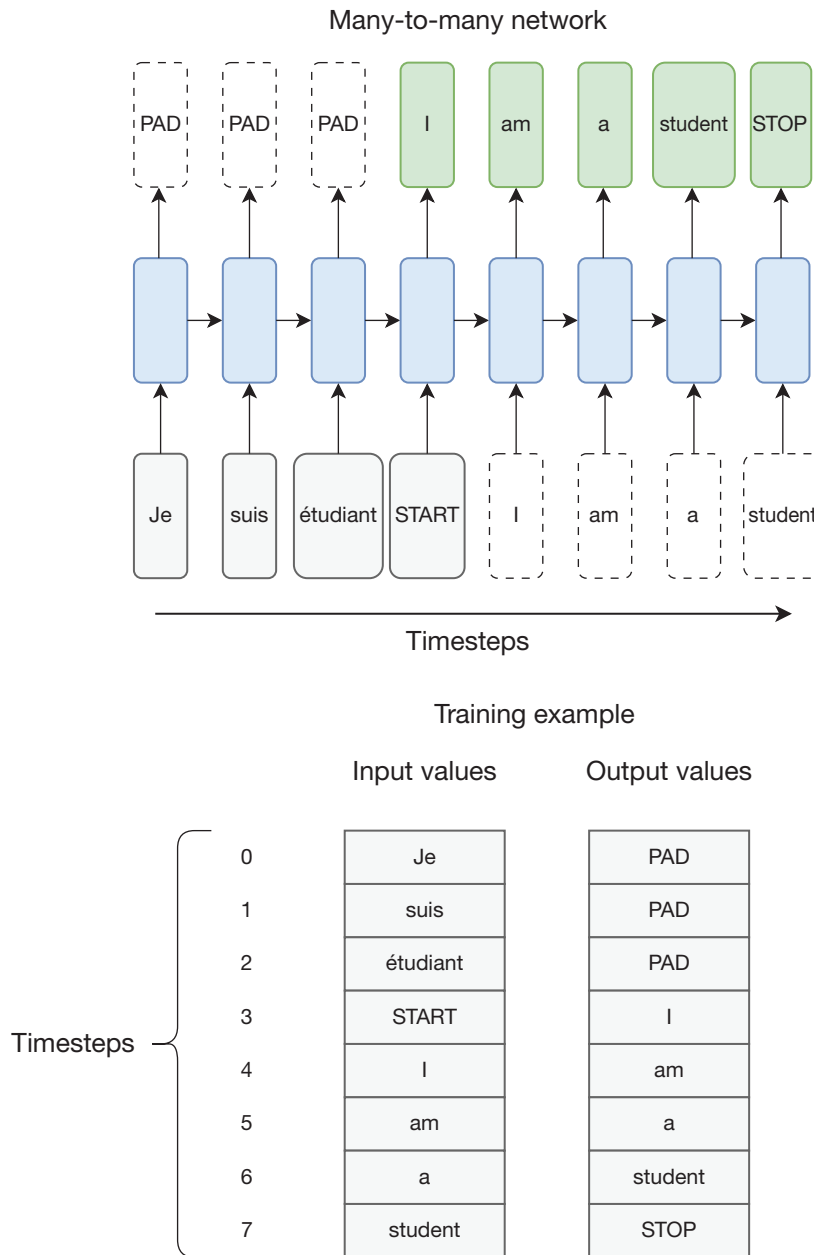
Figure 14-1 Neural machine translation is an example of a many-to-many sequence where the input and output sequences are not necessarily of the same length.
