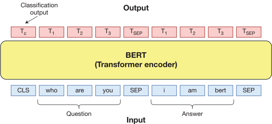
Figure D-5 BERT inputs and outputs. The input begins with a special classification CLS token. It is followed by a sequence of question tokens and a sequence of answer tokens. Each of those two groups ends with a special separation SEP token.
