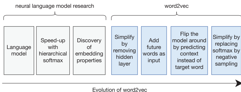
Figure 13-6 Evolution of neural language models into word2vec
