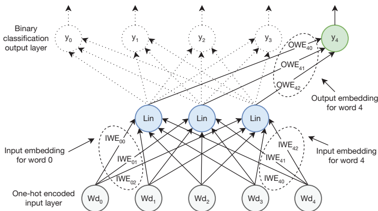
Figure 13-4 The word2vec continuous skip-gram model
