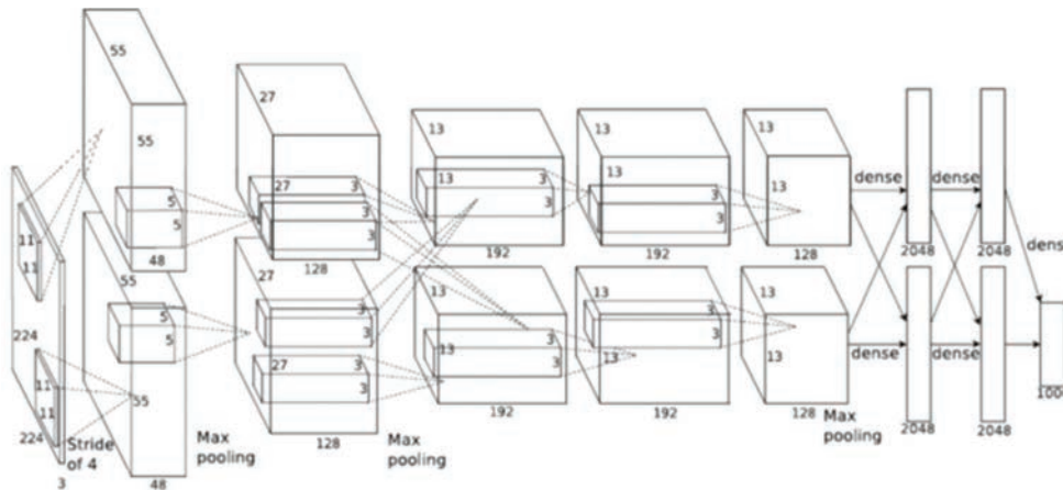
Figure 7-1 Topology of the AlexNet convolutional network. (Source: Krizhevsky, A., Sutskever, I., and Hinton, G., “ImageNet Classification with Deep Convolutional Neural Networks,” Advances in Neural Information Processing Systems 25 [NIPS 2012], 2012.)
