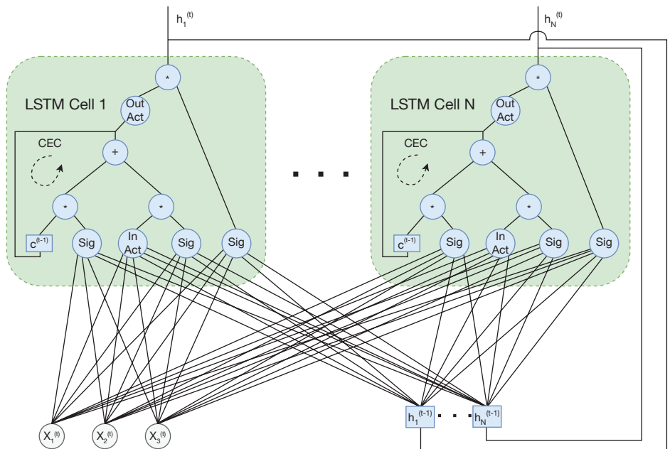
Figure H-1 Network of LSTM cells
