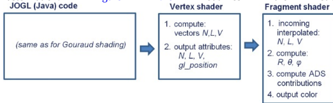
Figure 7.10 Implementing Phong shading.
