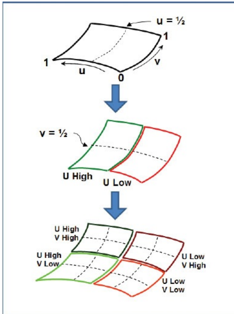
Figure 11.11 Recursive subdivision for Bézier surfaces.
