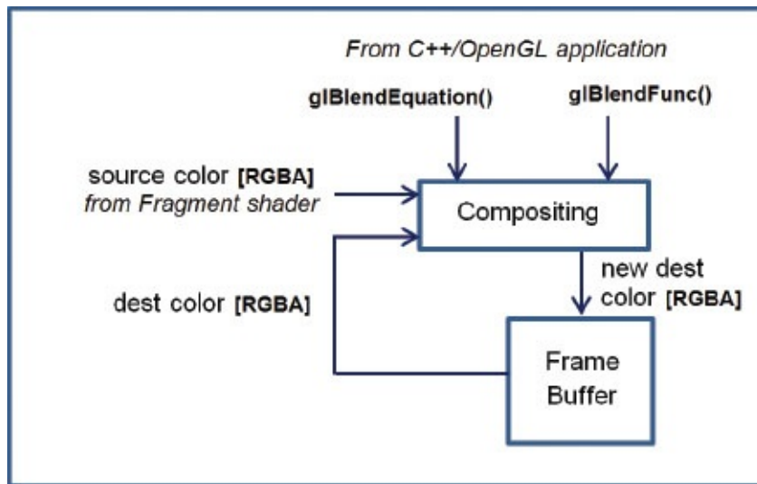
Figure 14.3 OpenGL compositing overview.
