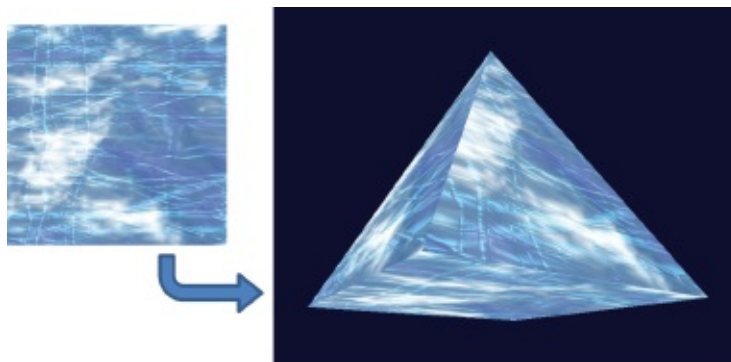
Figure 5.5 Pyramid texture mapped with “ice” image.
