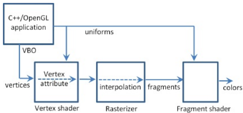
Figure 4.5 Data flow through Program 4.1.
