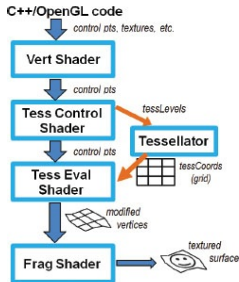
Figure 12.4 Overview of tessellation for Bézier surfaces.
