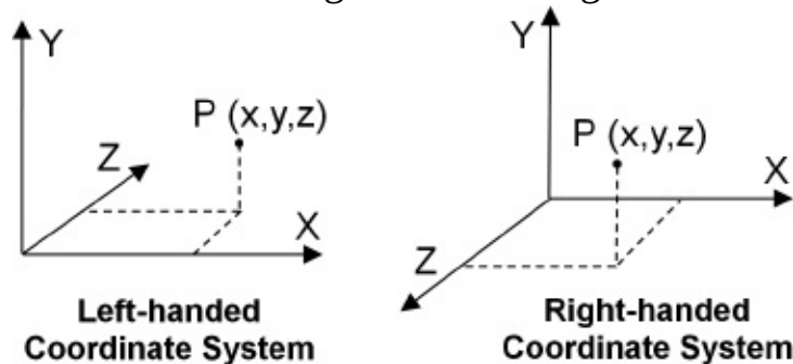
Figure 3.1 3D coordinate systems.
