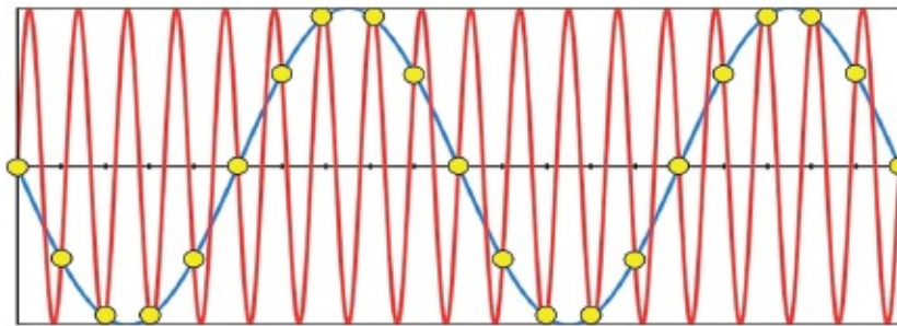
Figure 5.6 Aliasing due to inadequate sampling.
