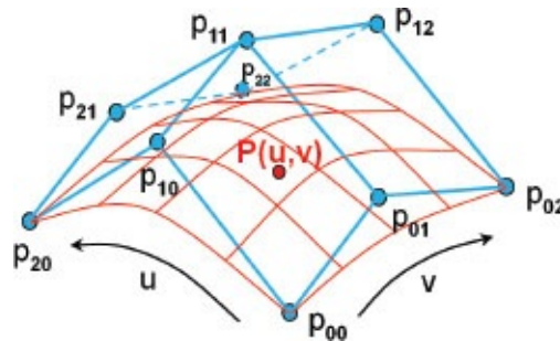
Figure 11.9 Quadratic Bézier control mesh and corresponding surface.
