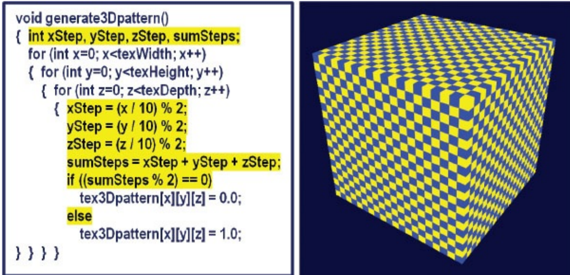
Figure 14.10 Generating a checkerboard 3D texture pattern.
