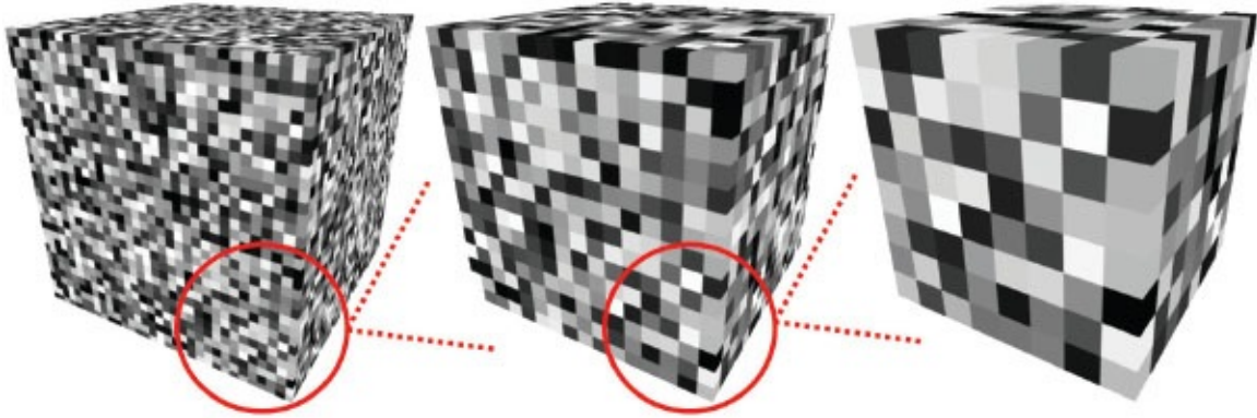
Figure 14.13 “Blocky” 3D noise maps with various “zooming in” factors.
