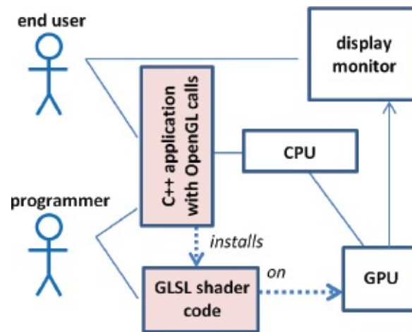
Figure 2.1 Overview of a C++-based graphics application.
