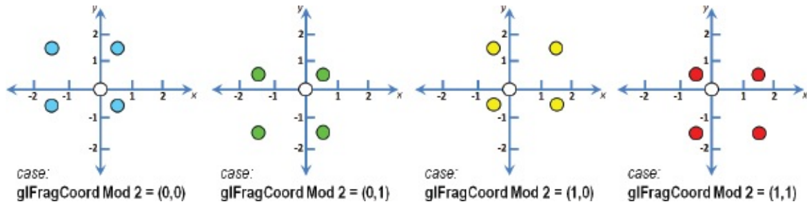
Figure 8.22 Dithered four-pixel PCF sampling cases.
