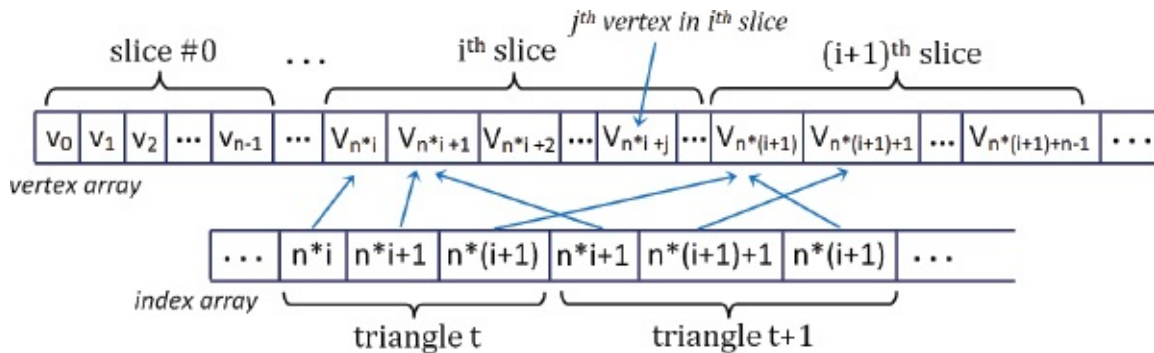
Figure 6.7 Vertex array and corresponding index array.
