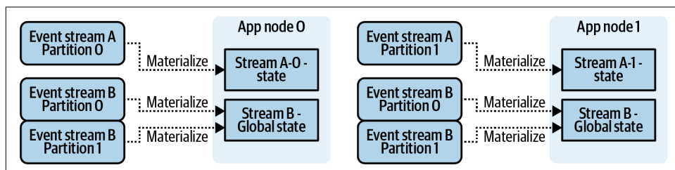
Figure 7-4. Global materialized state and nonglobal materialized state
