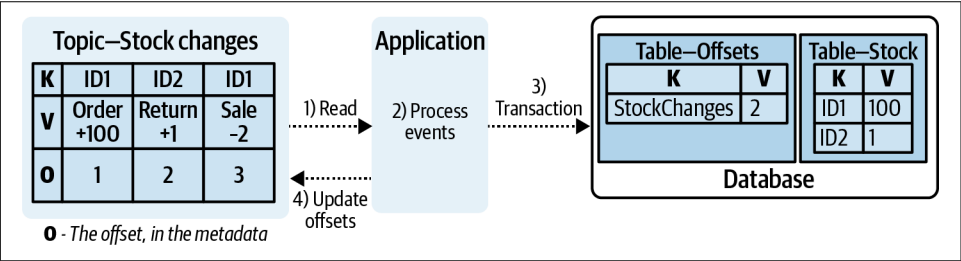
Figure 7-13. Normal transactional processing of events
