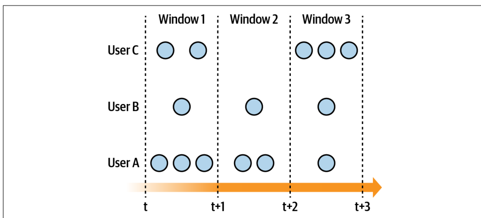
Figure 6-10. Tumbling windows
