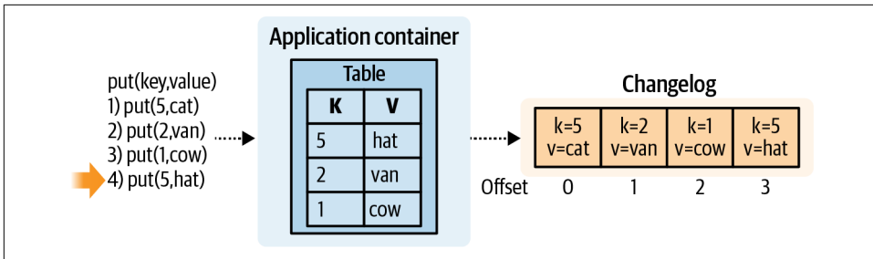
Figure 7-2. A state store with changelogging enabled
