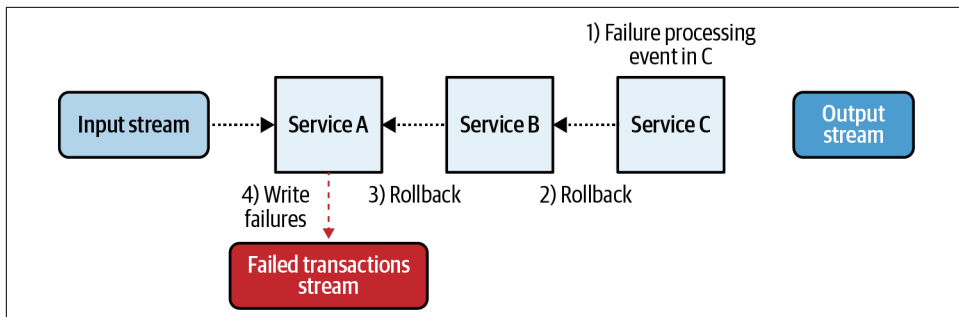
Figure 8-6. Choreographed transaction failure with rollbacks
