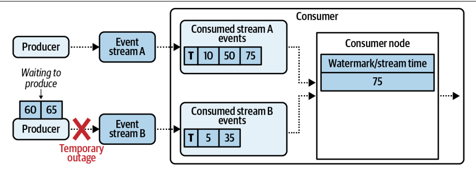
Figure 6-14. Temporary producer/broker connection outage
