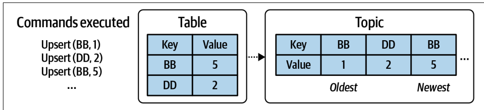
Figure 2-4. Generating an event stream from the changes applied to a table
