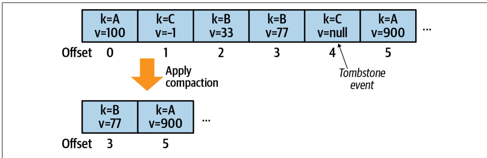
Figure 2-5. After a compaction, only the most recent record is kept for a given key—all tombstone records and their predecessors of the same key are deleted
