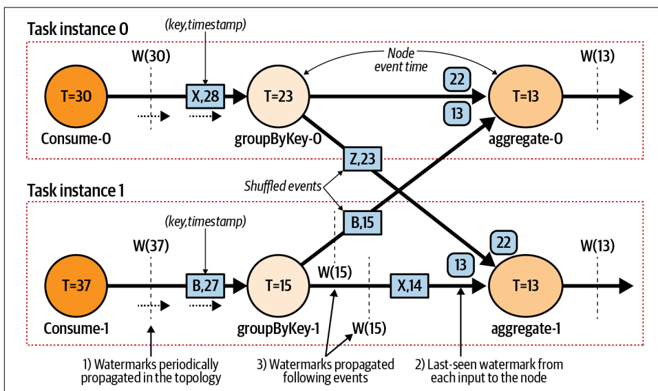
Figure 6-4. Watermark propagation between nodes in a single topology with multiple processors
